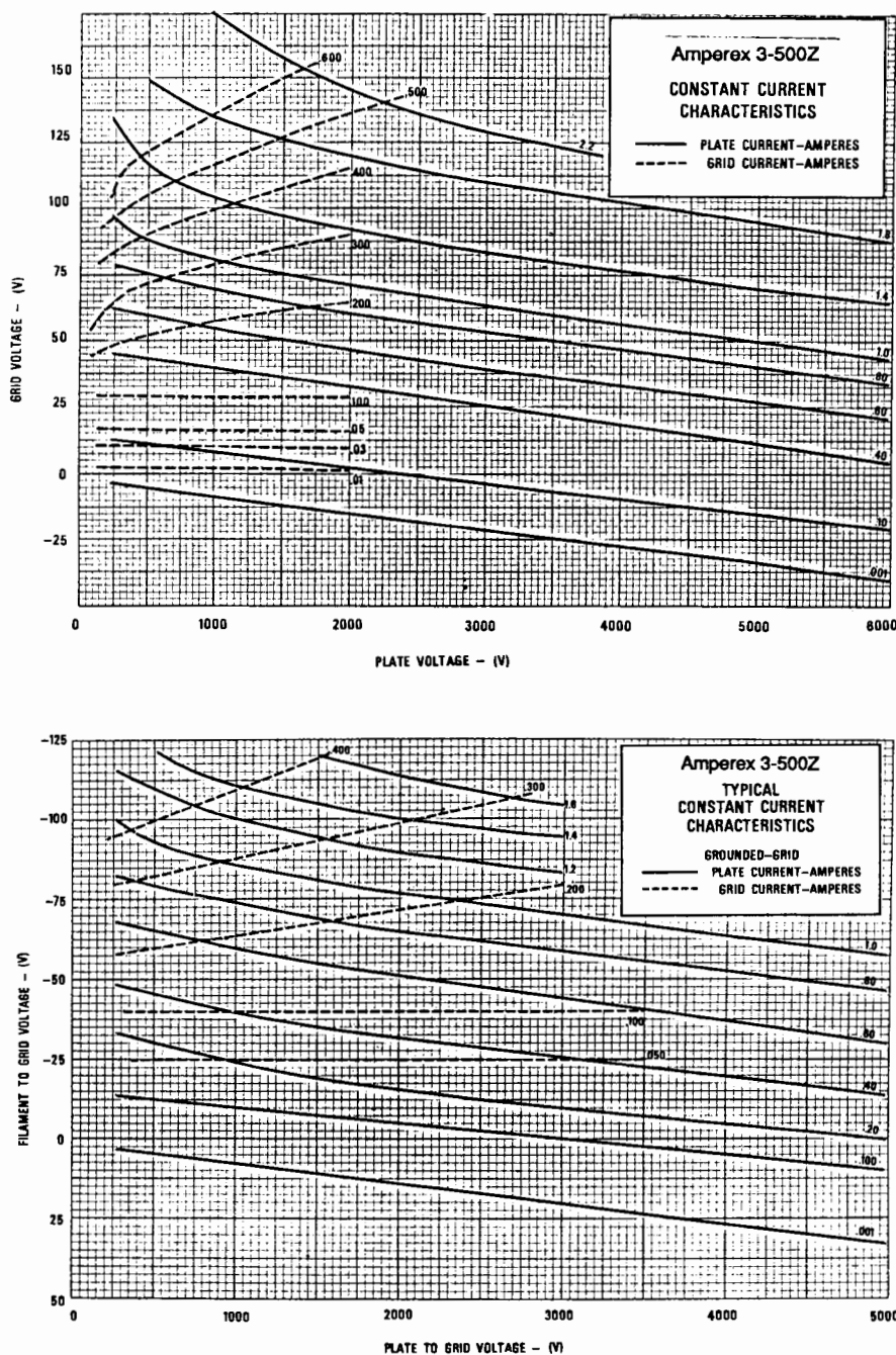
Figure 2 - Constant Current Characteristics
