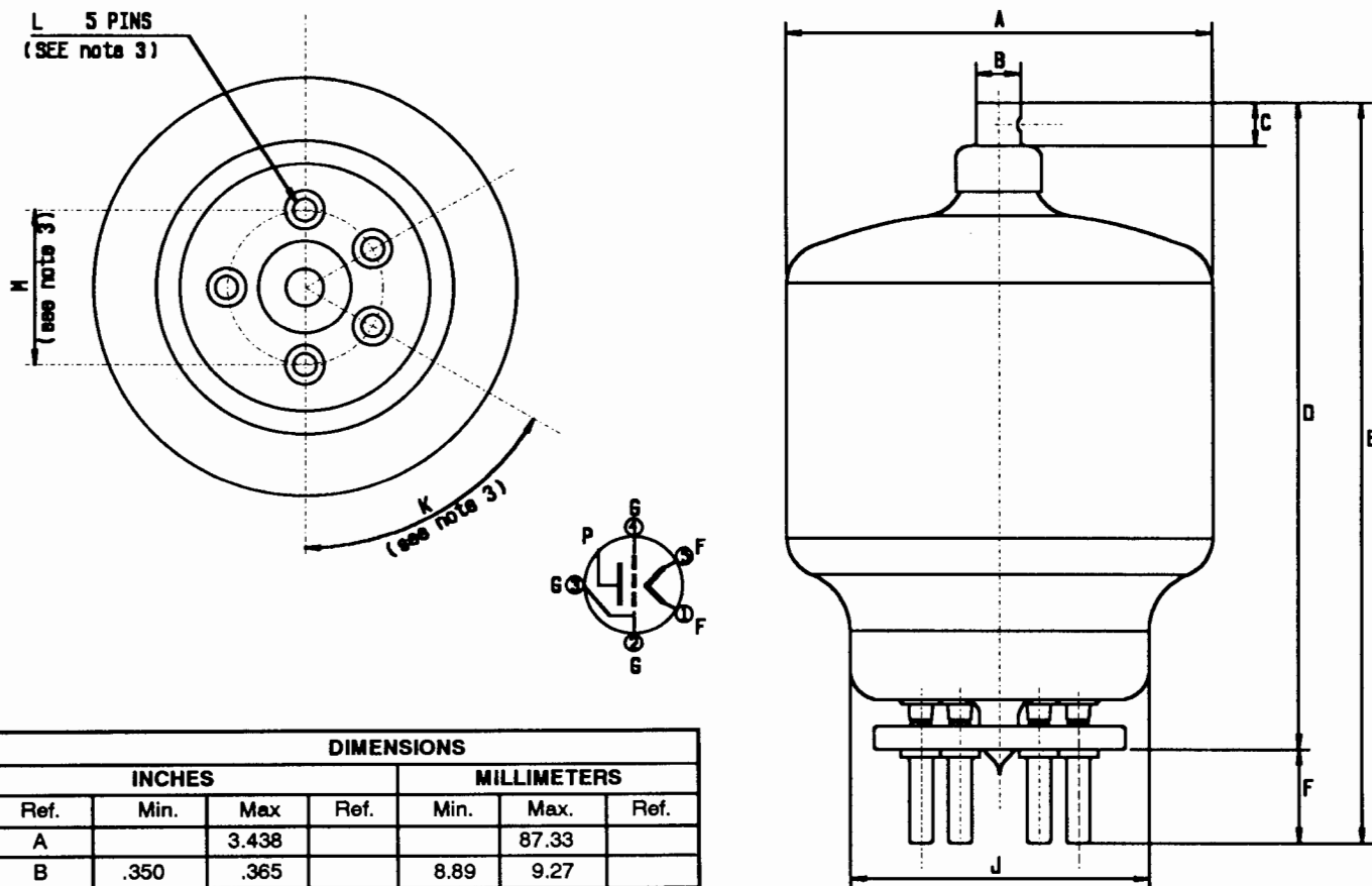
Figure 1 - Mechanical Outline
