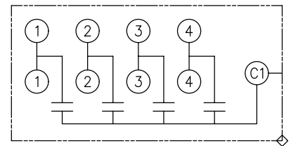
SCHEMATIC DIAGRAM - 411
