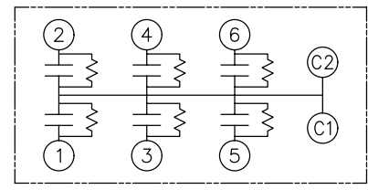
SCHEMATIC DIAGRAM - 617
