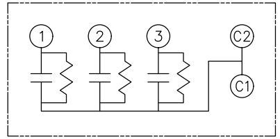
SCHEMATIC DIAGRAM - 327
