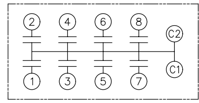
SCHEMATIC DIAGRAM - 800
